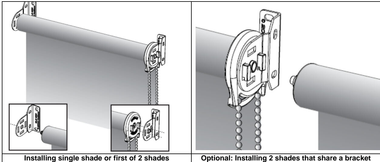
Installing single shade or first of 2 shades
